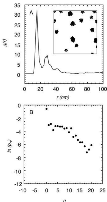
FIGURE 9 Effect of NF–NF attractive interactions on structure in NF distributions: strong cross bridging. When the NF–NF attractive energy is increased beyond 70\text{--}80kT , an abrupt phase transition occurs, leading to characteristic changes in the RDF and OPD. (A) RDF for attractive component of 150kT . Inspection of a sample configuration ( inset ) reveals NF–NF aggregation and phase separation. (B) OPD for the same pair potential. The pronounced maximum at n = 0 and the non-Gaussian shape reflect the large void spaces induced by NF–NF aggregation.
